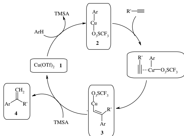
Figure 1. Plausible mechanism.
